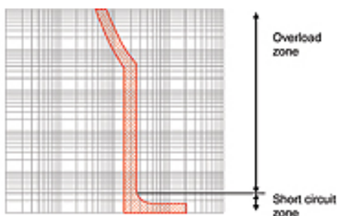
Figure 1 – A Typical Circuit Breaker Time-Current Curve
