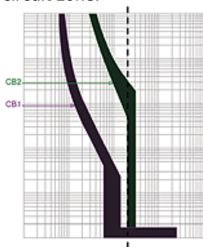
Figure 2 – Typical Circuit Breakers Selective Coordination Study
